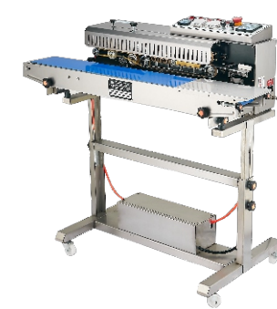
FRD1000NV/S & SF150NV/S Vacuum & Nitrogen Filling Band Sealer 真空充气印字封口机 Sealing Width/封口宽度: 10mm Sealing Speed/封口速度: 0-24m/min. Available Nitrogen Filling function only or Vacuum Sealer Only or Vacuum & Nitrogen Filling both. 可选择单充气、单真空或真空充气功能。
