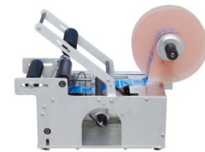
MT50 Round Bottle Labeling Machine 半自动圆瓶贴标机 Suitable Bottle Diameter: 18-120mm Label Size: L30-290mm W20-150mm Label Roller Diameter: 260mm Options: Label Width 250mm (MT50W) & Printing Function (MT50C)
