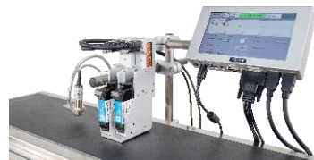
T220E Online Inkjet Printer 在线喷码机 Printing Font Height/字体高度: 1.5-12.7mm Max. Printing Lines/最大行数: 6 lines Screen Size/屏幕尺寸: 7 inch Available 40type of languages Options 2heads with 25.4mm Font Height
