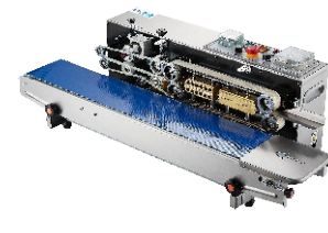
FRD1000W/S20 & FRD1000W/S27 Solid-Ink Coding Band Sealer 墨轮印字封口机 (宽封口) Sealing Width/封口宽度: 20mm & 27mm Sealing Speed/封口速度: 0-24m/min. Conveyor Width/输送台宽度: 150mm
