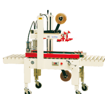
AS523 Carton Sealing Machine 半自动封箱机 Power Supply/供给电源: 110V,220-240V/50-60Hz Power/功率: 240W Conveyor Speed/输送速度: 20m/min Max. Carton Size/最大纸箱尺寸: W500xH520mm Min. Carton Size/最小纸箱尺寸: W100xH80mm Width Of Tape/胶带宽度: 50mm or 60mm Option: 3inch tape & overlap (Model AS523/31)
