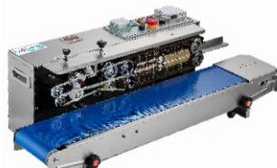
FRD1000W/SC (With Counter) Solid-Ink Coding Band Sealer 墨轮印字连续封口机 (计数型) Sealing Width/封口宽度: 10mm Sealing Speed/封口速度: 0-24m/min. Conveyor Width/输送台宽度: 150mm Printing letter/印字数: 2 lines 15 letters
