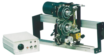
HP241 Color Ribbon Hot Printer 色带热打码机 Max. Printing Line/最多印字符数: 3 lines 12 letters Color Ribbon Width: 25/30/35mm Frame size/框架尺寸: 400/500/600mm
