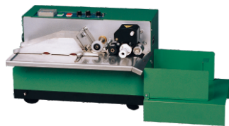
MY380F Solid-ink Coding Machine 固体墨轮标示机 Max. Printing Line/最多印字符数: 11 lines 10letters(T type letter) 8 lines 8letters ( R type letter) Max. Object Size/最大印物尺寸: L45-500mm W30-190mm
