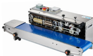
FRD1000W/SO (Opposite Direction) Solid-Ink Coding Band Sealer 墨轮印字连续封口机 (反向型) Sealing Width/封口宽度: 10mm Sealing Speed/封口速度: 0-24m/min. Conveyor Width/输送台宽度: 150mm Printing letter/印字数: 2 lines 15 letters
