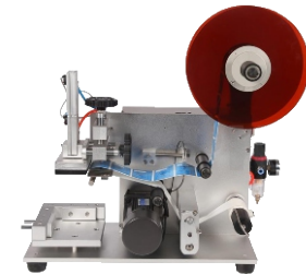
MT60 Semi-auto. Flat Labeling Machine 半自动平面贴标机 Suitable Product Height: 2-80mm Label Size: L30-80mm W30-80mm Label Roller Diameter: 260mm Options: Printing Function (MT60C)
