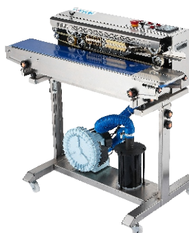
SF150G/P & SF150G/S Continuous Gas Filling Band Sealer 充气封口机 Sealing Width/封口宽度: 10mm Sealing Speed/封口速度: 0-24m/min.
