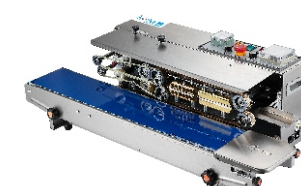
FRD1000W/SL Solid-Ink Coding Band Sealer 墨轮印字封口机 Sealing Width/封口宽度: 10mm Sealing Speed/封口速度: 0-24m/min. Conveyor Width/输送台宽度: 150mm Distance from bag mouth to sealing 70mm
